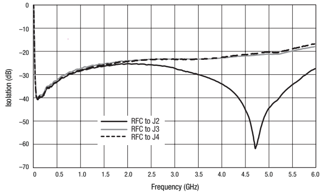
Figure 4. Isolation vs Frequency (RFC to J1 Insertion Loss State)
