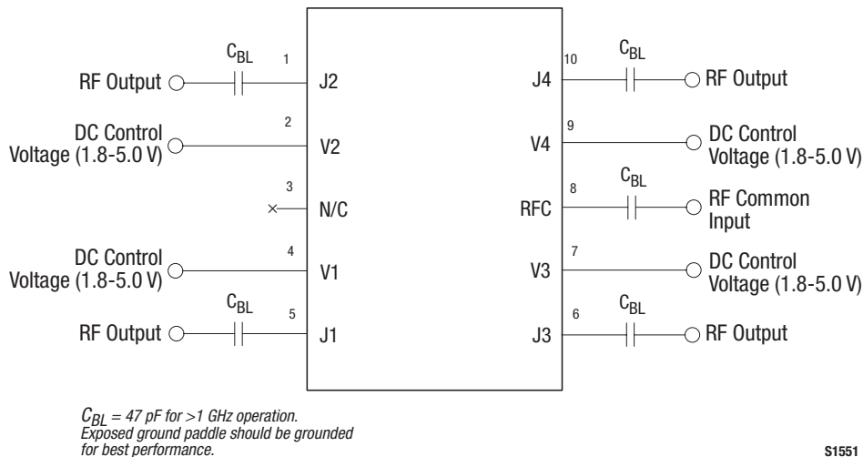
Figure 9. SKY13322-375LF Evaluation Board Schematic
