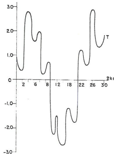
FIG. 16. The acoustic torque T per unit length on a strip of width 2a as a function of ka for \alpha=\pi/4 ( 45^\circ ). The vertical scale is the same as in Fig. 15.
