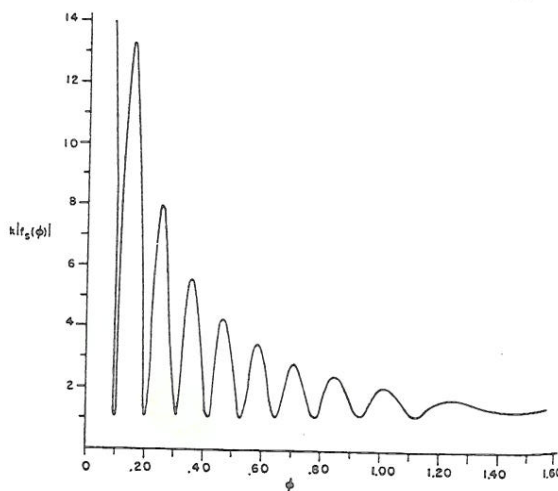
FIG. 5. The far-field diffraction pattern of a slit of width 2a hit normally by a plane wave; ka=10\pi . The curve, based on Eq. (6), results from single diffraction for a screen on which u=0 or \partial u/\partial n=0 . The ordinate is k|f_s(\varphi)| and the abscissa is \varphi in radians. The value at \varphi=0 is finite but too high to be shown.
