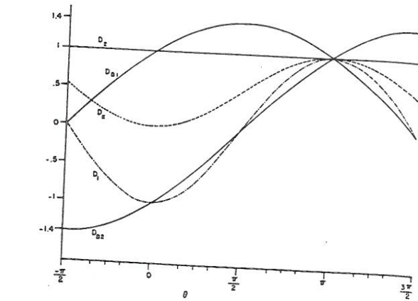
FIG. 14. Comparison of the Kirchhoff edge-diffraction coefficients D_1 , D_2 , and D_k with the Braunbek coefficients D_{B1} and D_{B2} for normal incidence ( \alpha=0 ). The latter coincide with our D_1 and D_2 given by Eq. (2) with the upper and lower signs, respectively. D_1 and D_2 result from the two usual modifications of the Kirchhoff theory and D_k = \frac{1}{2}(D_1 + D_2) comes from the usual form of it. The ordinate is -2(2\pi k)^{1/2} e^{-i\pi/4} \sin\theta D and the abscissa is \theta . All the coefficients are singular on the shadow boundary \theta=\pi but the singular factor \sin\theta has been removed. The dark side of the screen is at \theta=3\pi/2 and the illuminated side at \theta=-\pi/2 .
