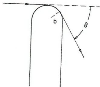
Fig. 18. Cross section of a screen of width 2b with a rounded end of radius b . A plane wave is normally incident upon it from the left. The dashed line is the shadow boundary. An incident ray which grazes the end of the screen is shown together with one of the surface diffracted rays which it produces in the shadow region. The angle between this ray and the shadow boundary is \theta .
