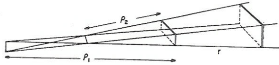
FIG. 9. A tube of rays and two small portions of wave fronts normal to them a distance \tau apart. The neighboring rays intersect at the two centers of curvature of the wave fronts. They are at the distances \rho_1 and \rho_2 from one wave front and at \rho_1 + \tau and \rho_2 + \tau from the other. The ratio of the areas of the wavefront sections is seen to be \rho_1 \rho_2 / (\rho_1 + \tau)(\rho_2 + \tau) .
