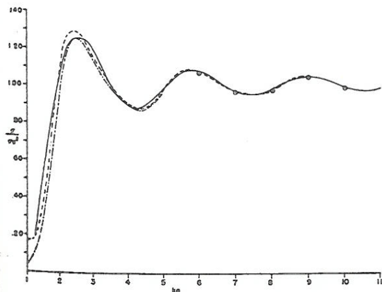
FIG. 11. The transmission cross section \sigma of a circular aperture of radius a in a thin screen on which u=0 . The wave is normally incident. The solid curve, based on Eq. (36), results from single and double diffraction; the dashed curve also includes all multiple diffractions. The dots and the broken curve up to ka=5 are based upon the exact solution of the reduced wave equation. 15 The ordinate is \sigma/\pi a^2 and the abscissa ka .
