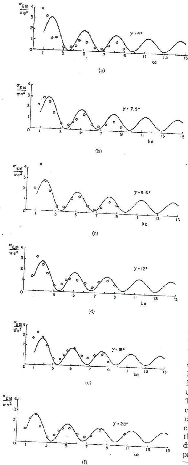
FIG. 13. Experimental and theoretical values of the electromagnetic back scattering cross section \sigma_{EM} of a finite circular metal cone for axial incidence. The ordinate is \sigma_{EM}/\pi a^2 and the abscissa is ka where a is the radius of the base of the cone. The circles are measured values and the curves are computed using the singly and doubly diffracted fields from the edge. The half-angle \gamma of the cone is indicated on each curve.
