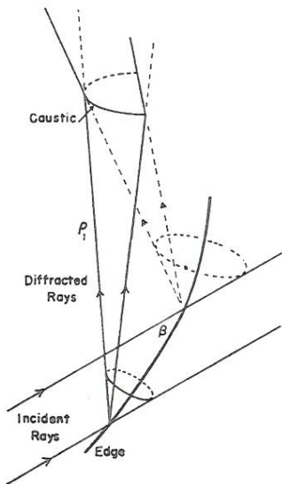
FIG. 8. A pair of neighboring incident rays hitting a curved edge, and some of the resulting diffracted rays. The two cones of diffracted rays intersect at the caustic, which is at the distance \rho_1 from the edge along the rays.
