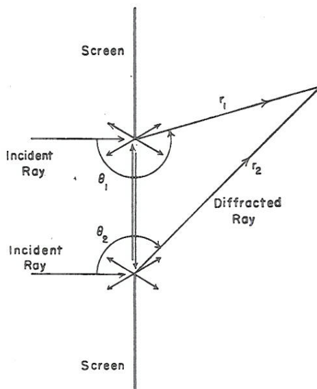
FIG. 3. The diffracted rays produced by a plane wave normally incident on a slit in a thin screen. The two incident rays which hit the slit edges are shown, with some of the singly diffracted rays they produce. One diffracted ray from each edge is shown crossing the slit and hitting the opposite edge, producing doubly diffracted rays.
