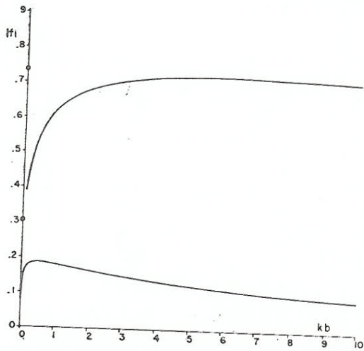
FIG. 21. The far-field amplitude |f(\pi/4, kb)| in the shadow of the screen of Fig. 18 in the direction \theta = \pi/4 as a function of kb . The curves are based upon the geometrical theory of diffraction while the points at kb=0 are determined from the solution for diffraction by a half-plane. The upper curve and point apply to a screen on which \partial u/\partial n=0 ; the lower ones to a screen on which u=0 . Probably only the decreasing portions of the curves are correct, and most likely the amplitude decreases monotonically for all values of kb .
