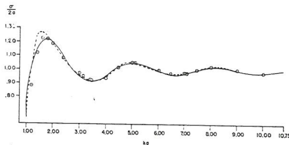
FIG. 6. The transmission cross section of a slit of width 2a as a function of ka , for normal incidence with u=0 on the screen. The solid curve, based on Eq. (10), results from single and double diffraction; the dashed curve includes single and all multiple diffraction. The dots are based upon the exact solution of the reduced wave equation with u=0 on the screen. 11 The ordinate is \sigma/2a and the abscissa is ka .
