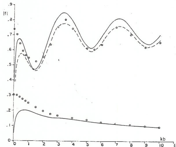
FIG. 20. The far-field amplitude |f(\pi/4, kb)| in the shadow of the screen of Fig. 19 in the direction \theta = \pi/4 as a function of kb . The upper curves and points apply to a screen on which \partial u/\partial n = 0 while the lower ones pertain to a screen on which u = 0 . The encircled points were obtained by laborious numerical computation of the series solution of the boundary-value problem; the curves were obtained from the formulas given by the geometrical theory of diffraction. The dashed curve was obtained from a formula in which an improved expression for \alpha was used.
