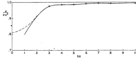
FIG. 12. The transmission cross section \sigma for normal incidence on a circular hole in a screen on which \partial u/\partial n=0 . The ordinate is \sigma/\pi a^2 and the abscissa is ka . The solid curve is based upon Eq. (40) which results from single and double diffraction. The encircled points and the dashed curve are the exact values computed by Bouwkamp. 13
