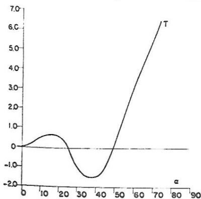
FIG. 15. The acoustic torque T per unit length on a strip of width 2a as a function of the angle of incidence \alpha for ka=5 . The vertical scale is the value of T|a^2P^2/\rho_0c^2\pi^{\frac{1}{2}}(ka)^{\frac{1}{2}}|^{-1} , where P is the amplitude of the incident pressure wave, \rho_0 is the density of the medium and c is its sound speed. The values of \alpha at which T=0 are equilibrium angles which are stable if T_\alpha < 0 and unstable if T_\alpha > 0 . The curve does not apply near \alpha=\pi/2 , which corresponds to grazing incidence, at which T=0 . T is an odd function of \alpha .
