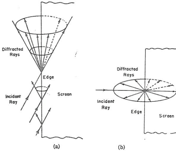
FIG. 1. (a) The cone of diffracted rays produced by an incident ray which hits the edge of a thin screen obliquely. (b) The plane of diffracted rays produced by a ray normally incident on the edge of a thin screen.
