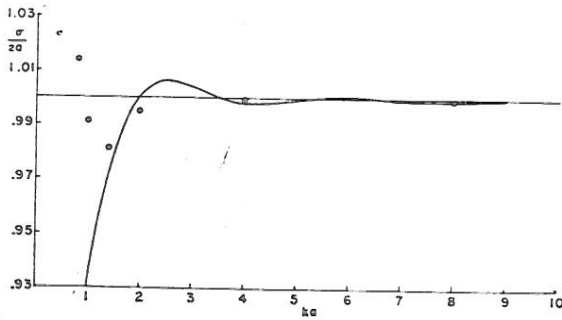
FIG. 7. The transmission cross section of a slit of width 2a as a function of ka , for normal incidence with \partial u/\partial n=0 on the screen. The curve, based on Eq. (16), results from single and double diffraction. The dots are based upon the exact solution of the reduced wave equation. 13 The ordinate is \sigma/2a and the abscissa is ka .
