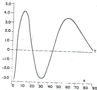
Fig. 17. The acoustic torque T on a circular disk of radius a as a function of the angle of incidence \alpha for ka=5 . The vertical scale is the value of T|P^2a^3/\rho_0c(ka)^2|^{-1} . P , \rho_0 , and c are defined in the caption of Fig. 15. The values of \alpha at which T=0 are equilibrium values, stable if T_\alpha < 0 and unstable if T_\alpha > 0 . The curve does not apply near \alpha=0 (normal incidence) nor \alpha=\pi/2 (grazing incidence).
