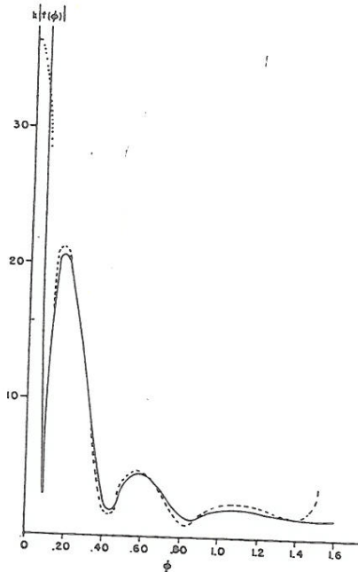
FIG. 10. The diffraction pattern of a circular hole of radius a hit normally by a plane wave; ka=3\pi . The solid curve, based on Eq. (25) results from single diffraction with either u=0 or \partial u/\partial n=0 on the screen. The dashed curve, for the case u=0 on the screen, also includes multiple diffraction. The dotted curve near \varphi=0 includes the caustic and shadow-boundary corrections given by (30).
