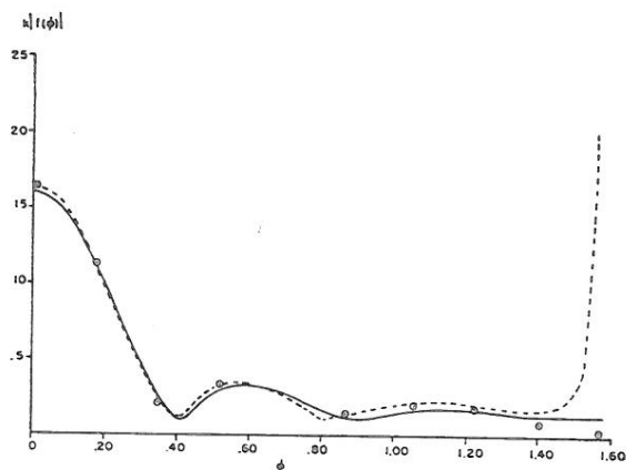
FIG. 4. The far-field diffraction pattern of a slit of width 2a hit normally by a plane wave; ka=8 . The solid curve based upon Eq. (6) results from single diffraction, and applies to a screen on which u=0 or \partial u/\partial n=0 . The dashed curve includes the effects of multiple diffraction for a screen on which u=0 . The dots are based upon the exact solution of the reduced wave equation for a screen on which u=0 . 11 The ordinate is k|f_s(\varphi)| and the abscissa is \varphi in radians.
